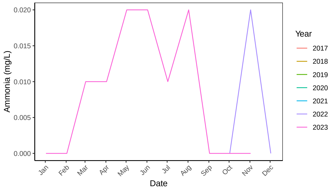
B2 Raceway 1 Ammonia (mg/L) Monthly Statistics
